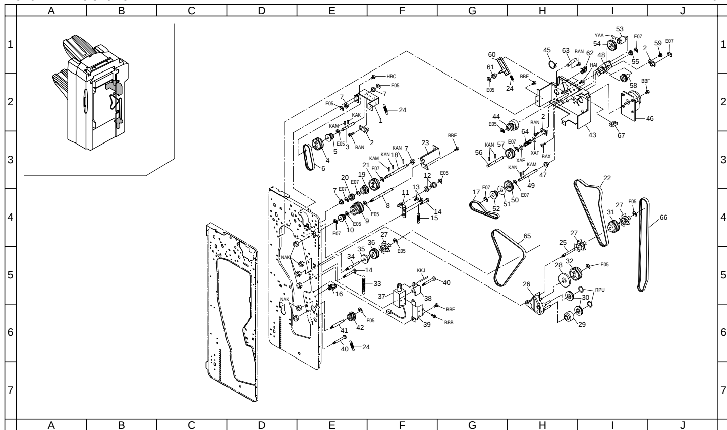
FIG. 8 DRIVING SECTION 1
