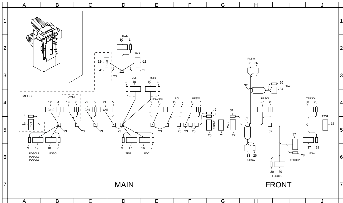
FIG. 11 ELECTRICAL COMPONENTS 2
