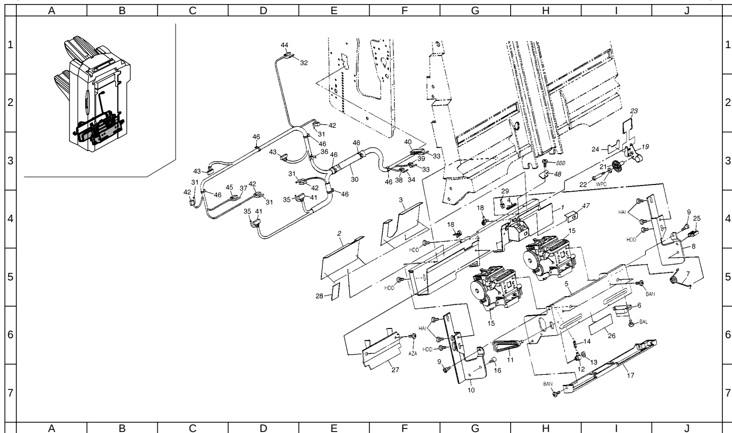
FIG. 7 MIDDLE TRAY 2
