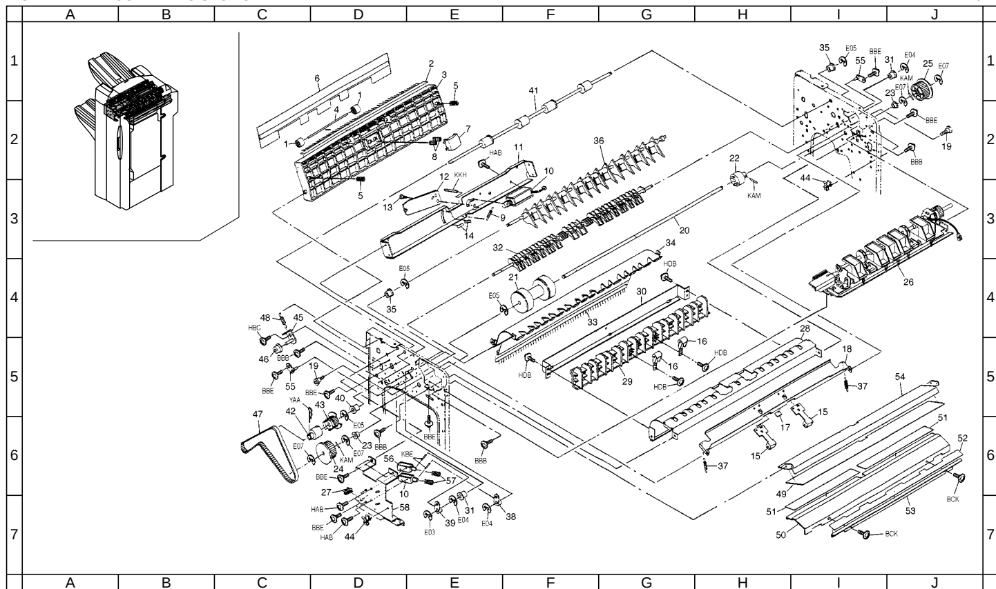
FIG. 4 PAPER CONVEYING SECTION 1
