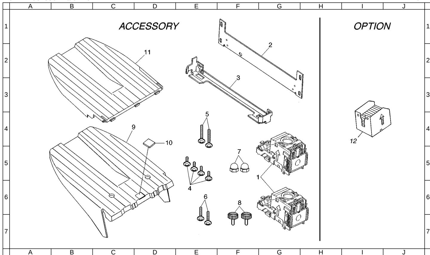
FIG. 12 ACCESSORY & OPTION
