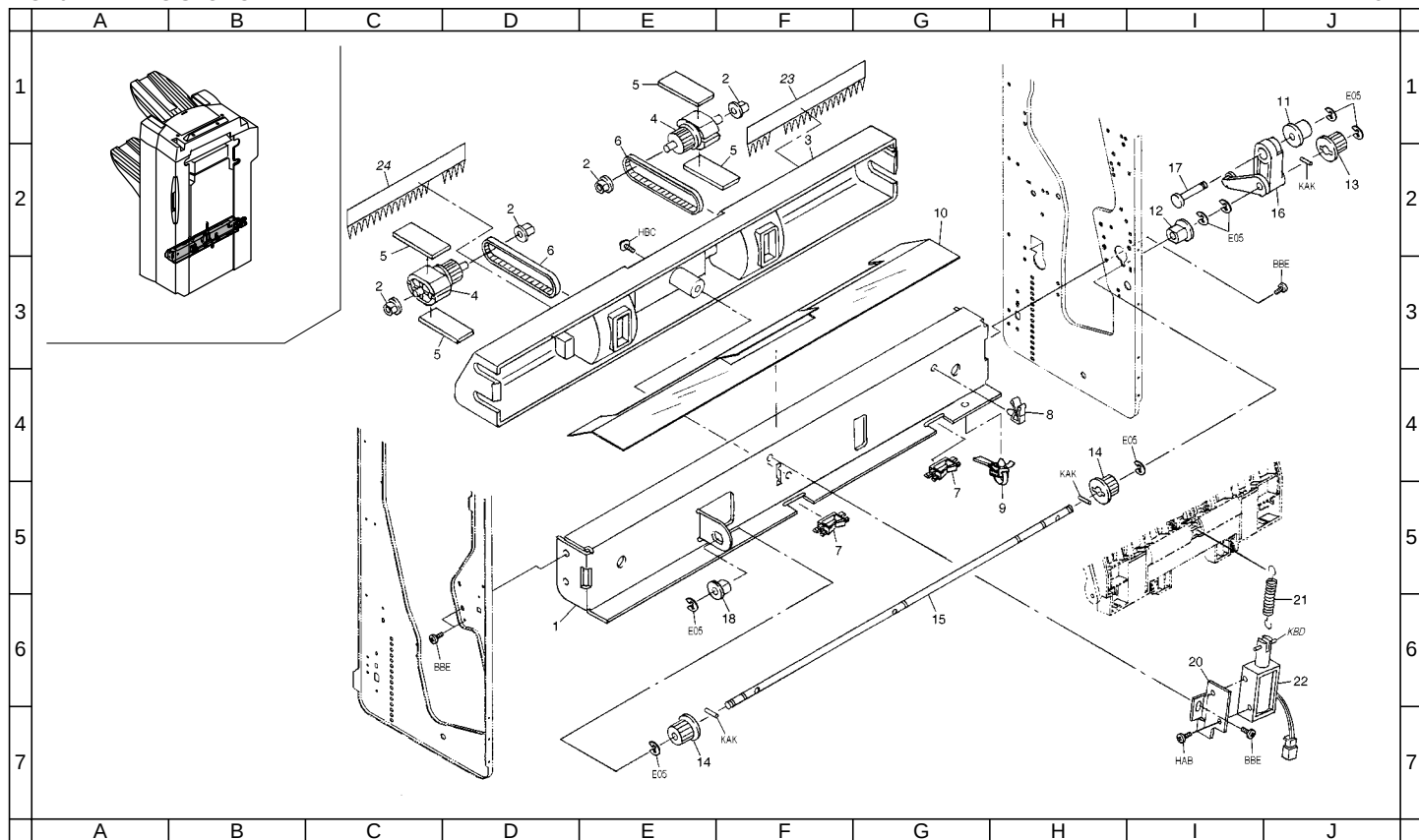
FIG. 9 DRIVING SECTION 2
